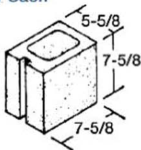
6x8x16 Combination Half Sash
